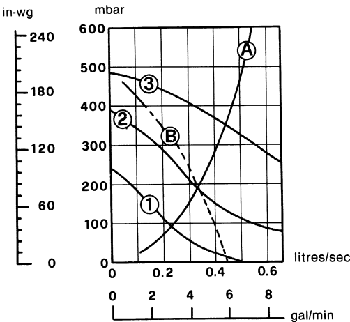
1 2 3 Speed settings A Boiler pressure drop B Max. available pump head C.H.
