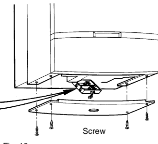
Fixing screw front
